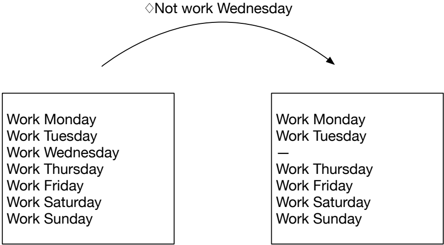
Figure 4: Removing propositions
