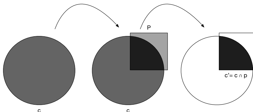
Figure 1: Stalnaker's picture
